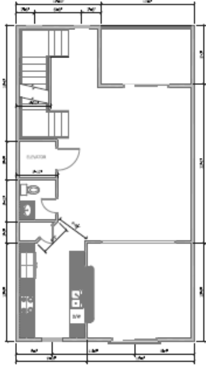
SECOND FLOOR PLAN 1/4" = 1'
