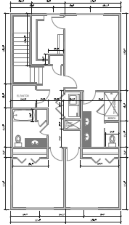
THIRD FLOOR PLAN 1/4" = 1'
